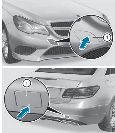
Towing eye covers (example: Coupe)
